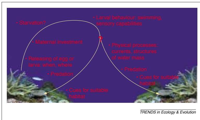
Fig. 1. Factors affecting larval dispersal. The path taken by a larva might lead to it returning to the natal reef or dispersing to a more or less distant site. The path taken is determined by a mix of factors, which act synergistically over the larval period to determine the dispersal of each member of a larval cohort. Where and when eggs or larvae enter the water column, their quality, and the food resources and predators that they encounter will affect survival, condition and growth rates. Condition and growth rates will determine the development of swimming and sensory abilities, and these will determine how larvae respond to the physical environment and to any cues from reefs. We can predict considerable variation among cohorts and locations in the paths travelled, as well as among species, but we cannot yet do much more. We lack information on most of the factors operating.
